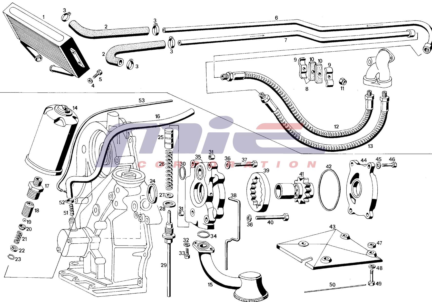
Tavola 5 - Pompa olio e filtro Table 5 - Oil pump and filter
