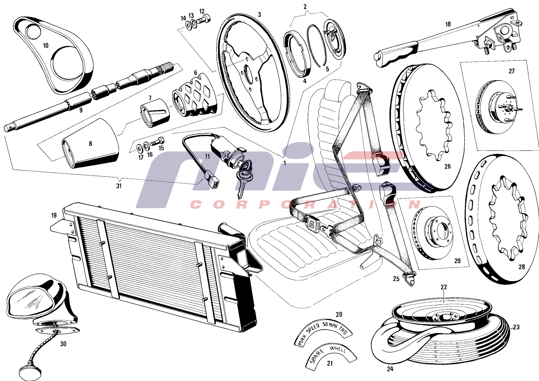
Tavola 6 - Piantone sterzo-radiatore-freni Tableau 6 - Direction - Radiateur - Freins Table 6 - Steryng - Engine cooling - Brakes Tafel 6 - Lenkung - Motorkühlung - Bremse
